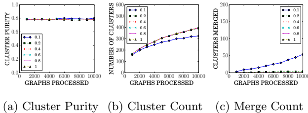
Figure 2: Effect of cluster merge threshold value on the CORA graph ( SoB size of 200).
