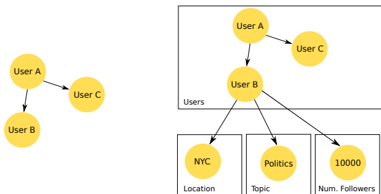
Figure 1: How graph augmentation enlarges the transaction graph G_t (left) to G_s (right). All of G_s (right) is the augmented subgraph.
