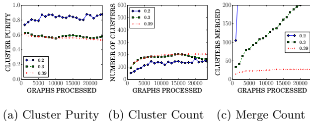
Figure 3: Effect of cluster merge threshold on the MSD graph ( SoB size of 200).
